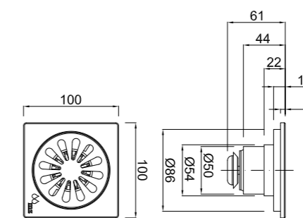
Sumidero inspeccionable 10 x 10 cm Ø 50 mm, con válvula antiretorno Self-closed floor drain, 10 x 10 cm, un- tireturn valve, Ø 50 mm Vidage Douche Encastré Reviewable
