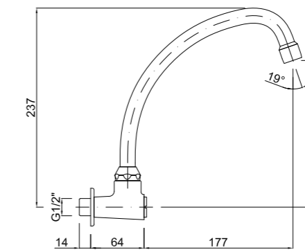
Caño tubo cisne 18 mm giratorio 1/2" 1/2" wall spout, "swan" model Bec mural 1/2" 18mm
