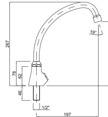
Caño tubo cisne 18 mm, 1/2" giratorio 1/2" tabletop spout, "swan" model Bec 1/2" 18mm
